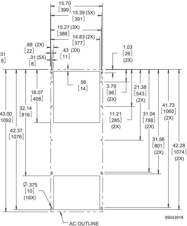
Cutout Dimensions (Internally Mounted)
