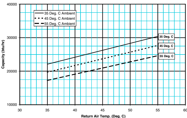
62-2226-xxx 60HZ CAPACITY CURVE
